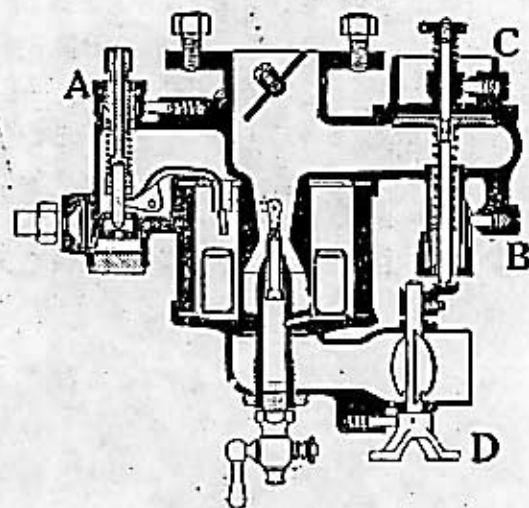
SECTIONAL VIEW
