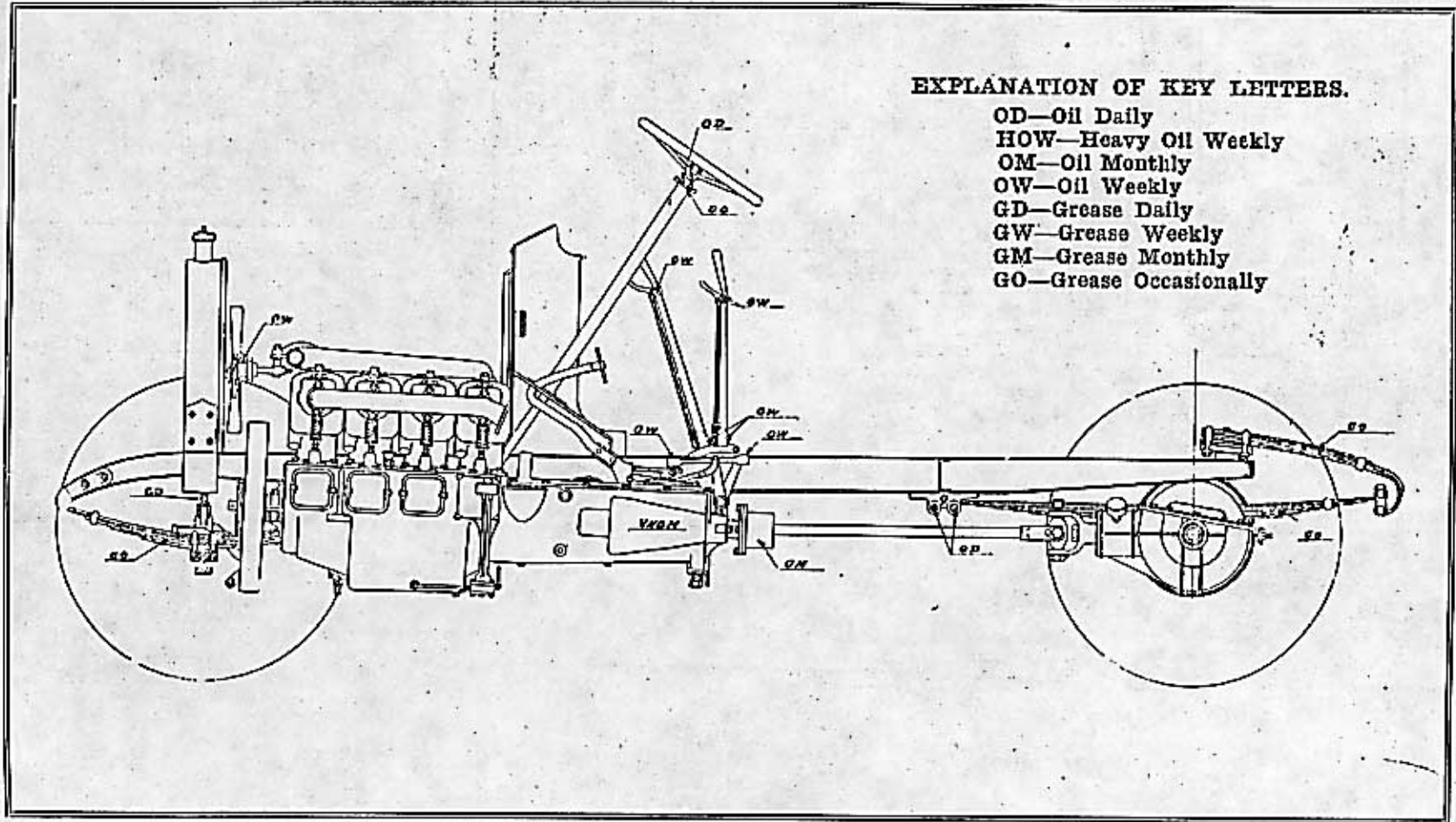
Lubricating Chart Maxwell Special, Side View
