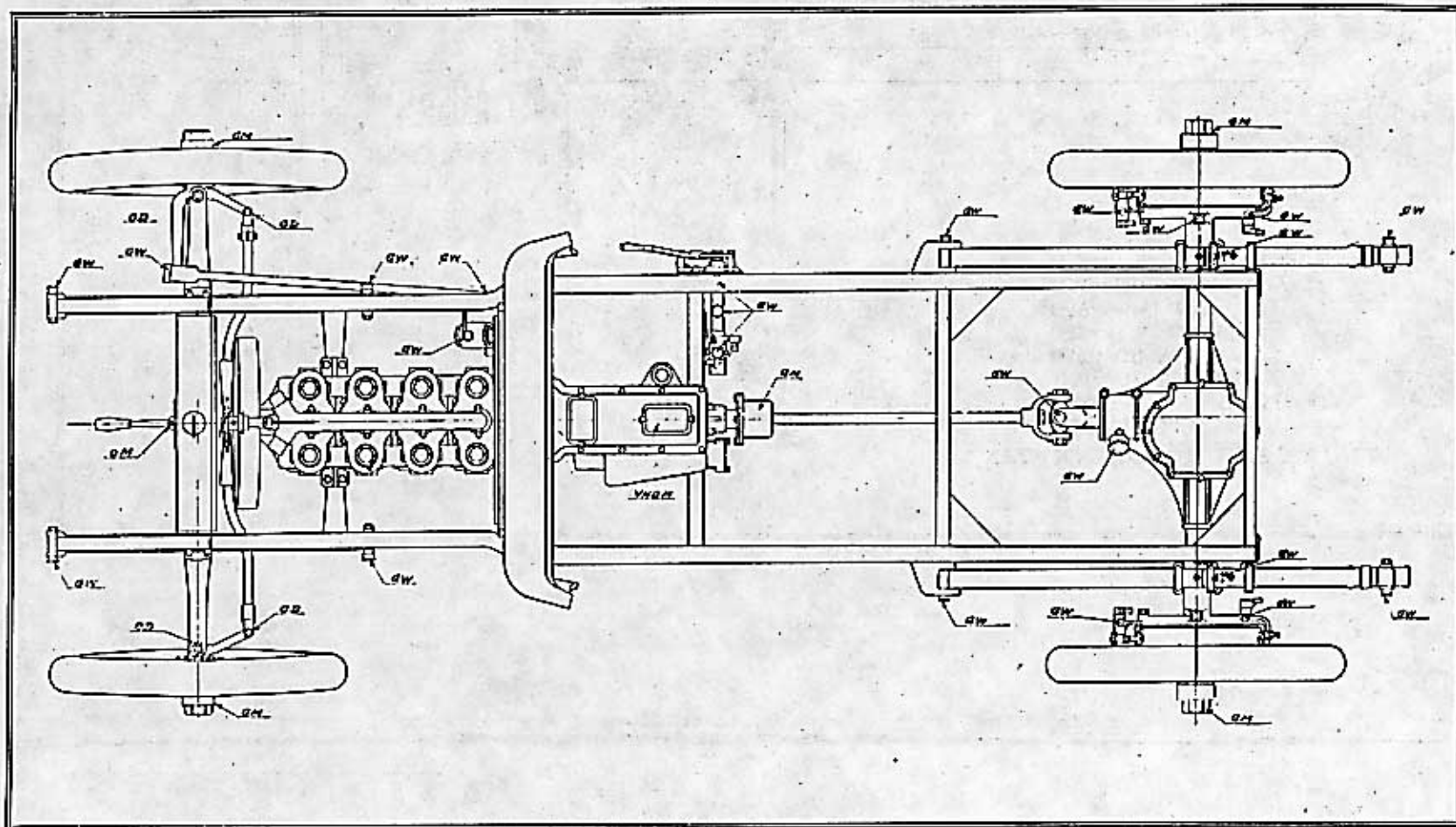
Lubricating Chart Maxwell Special, Top View
