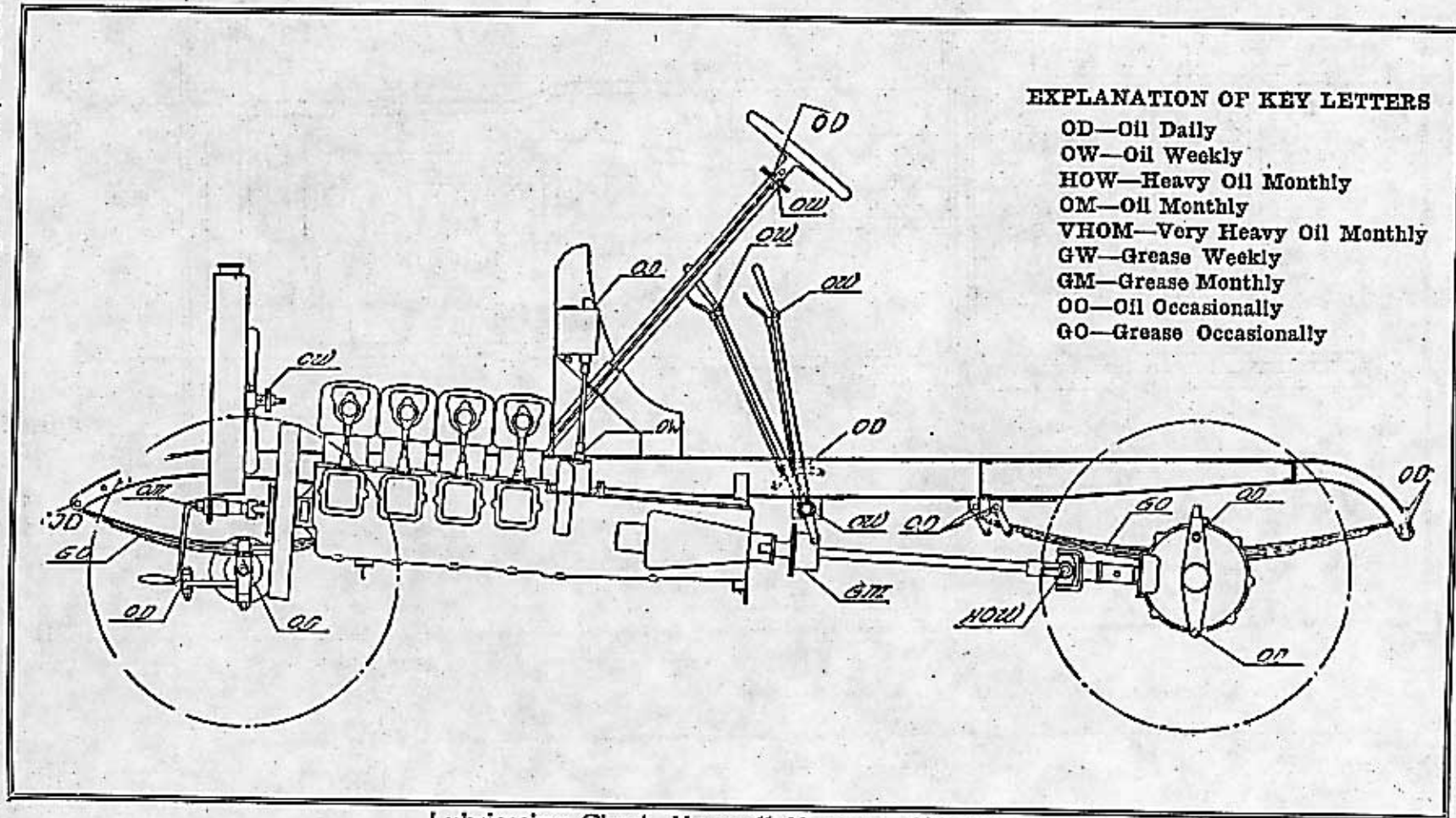
Lubricating Chart, Maxwell Mercury, Side View
