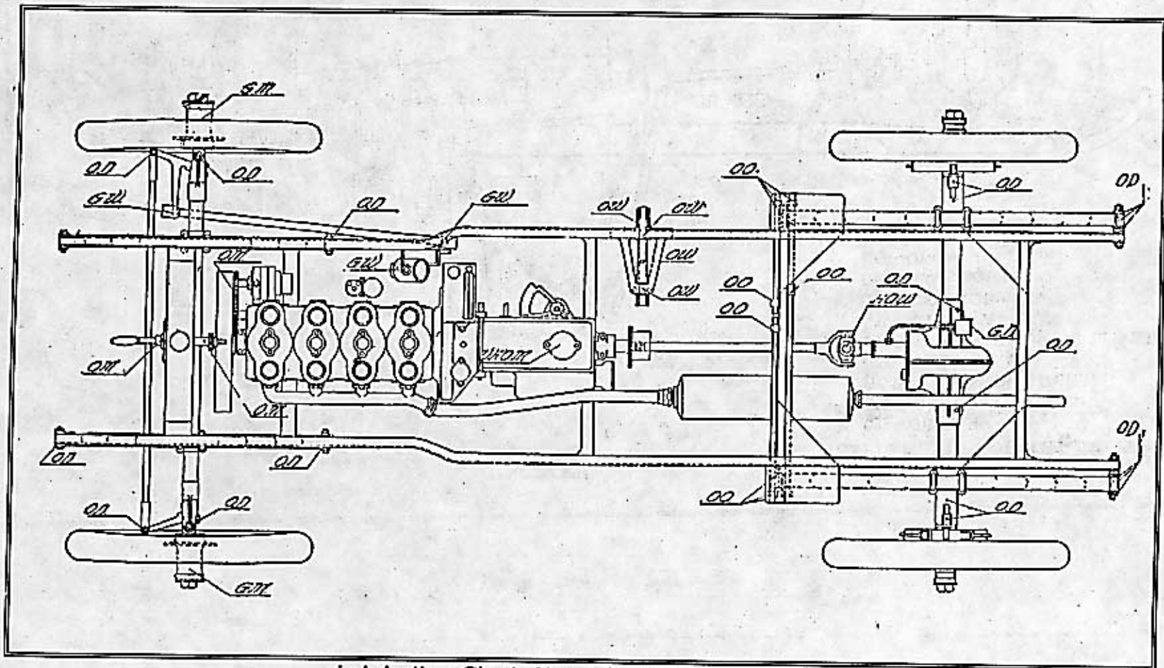
Lubricating Chart, Maxwell Mercury, Top View
