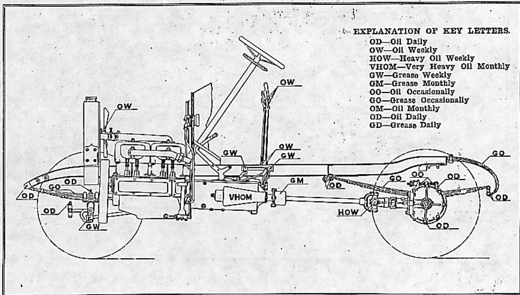
Lubricating Chart, Maxwell Mascotte, Side View
