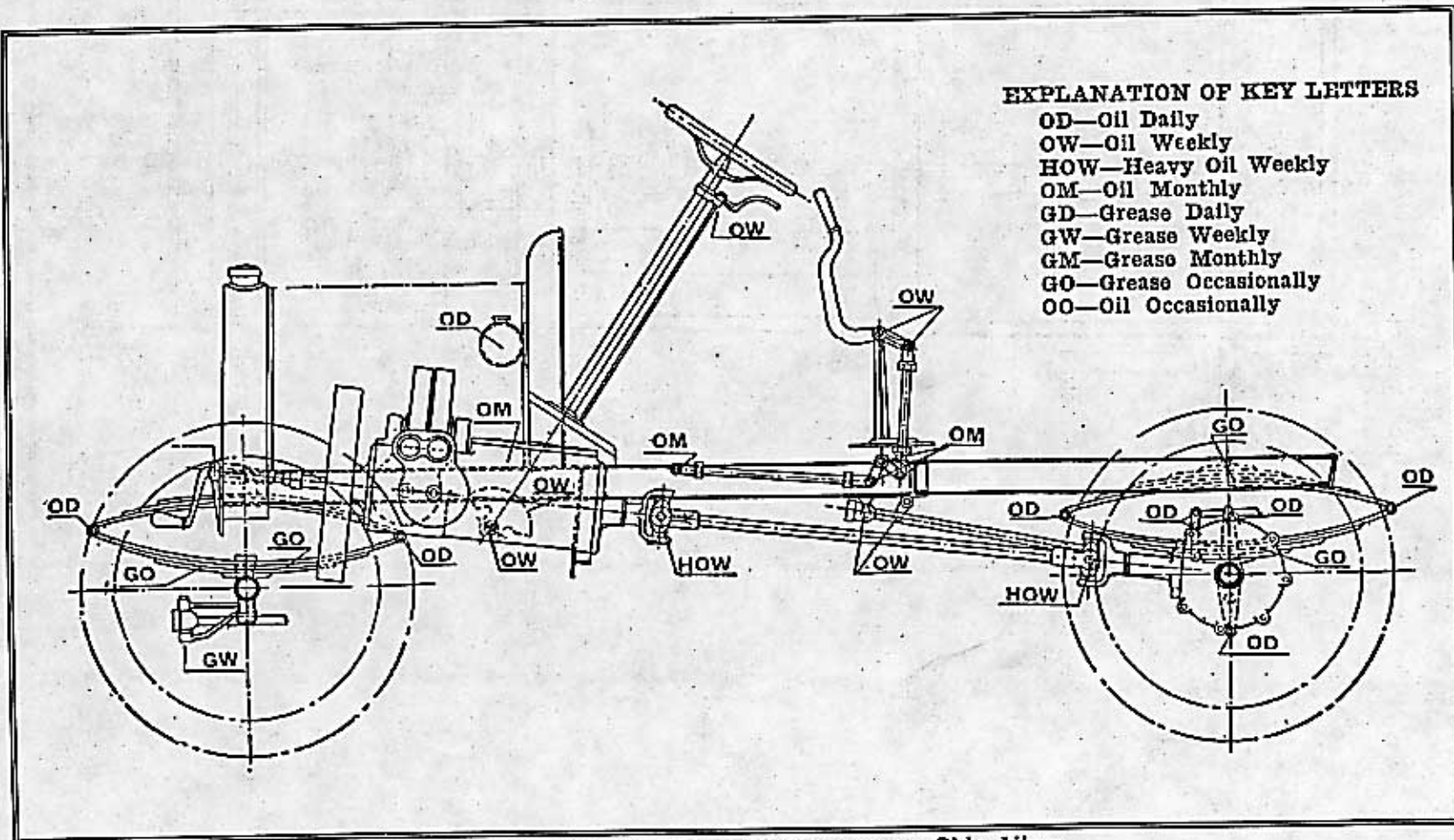
Lubricating Chart, Maxwell Messenger, Side View
