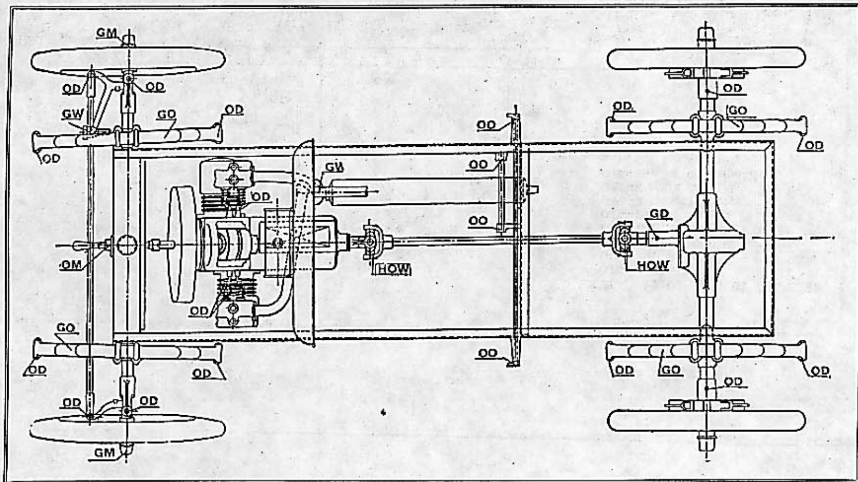
Lubricating Chart, Maxwell Messenger, Top View
